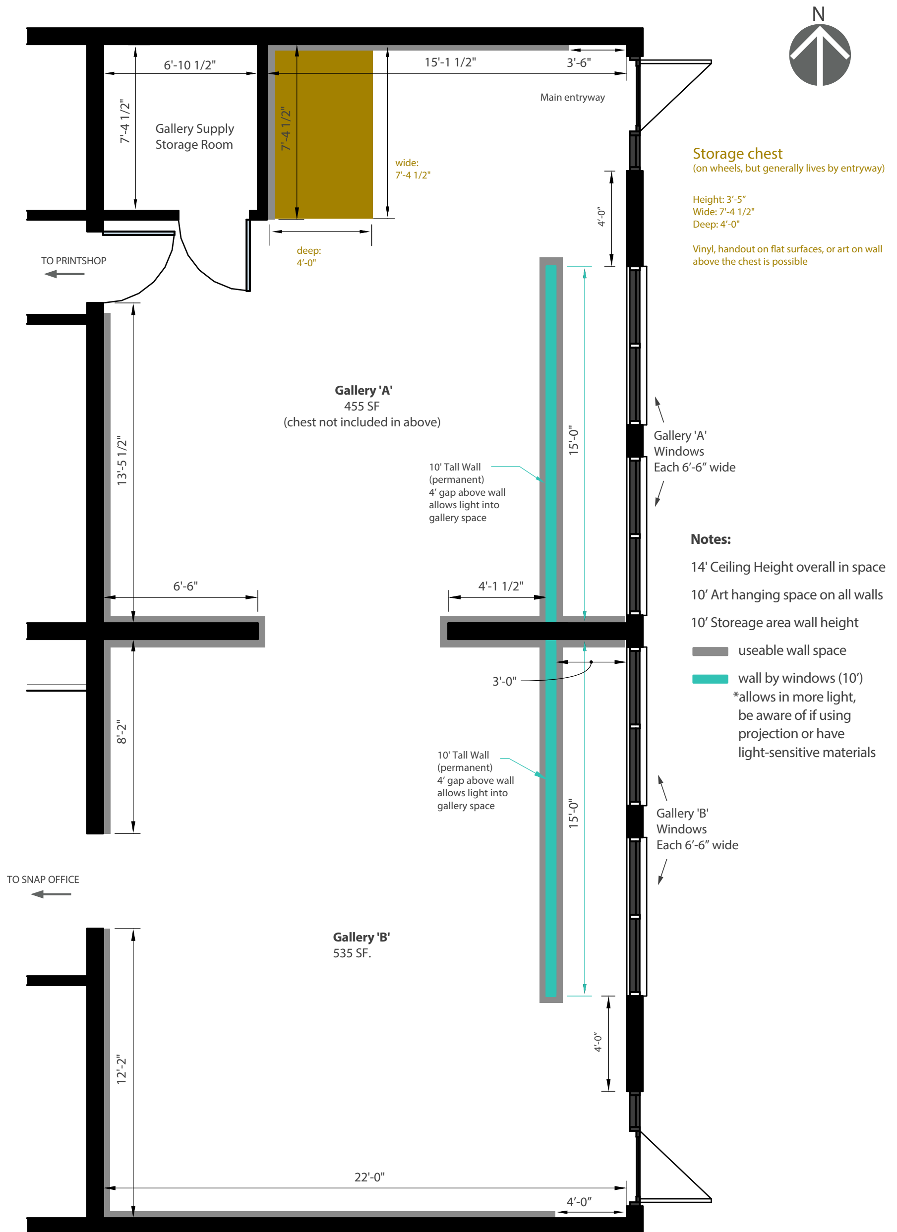
Key Plan
